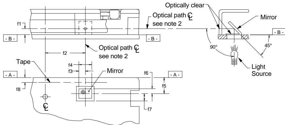
Calibration configuration
