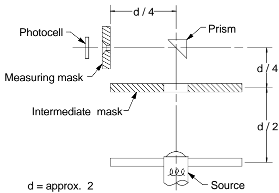
Calibration configuration
