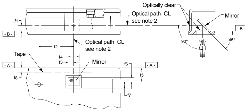
Calibration configuration
