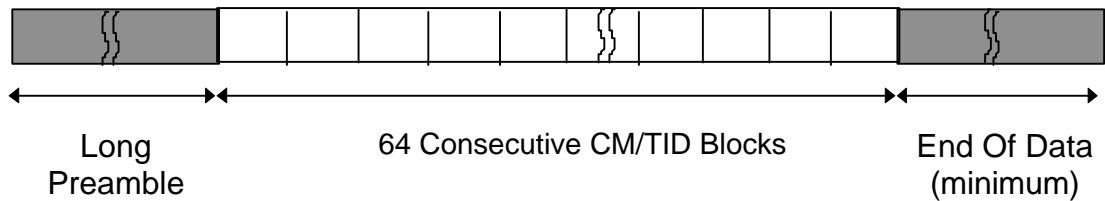
FIGURE B.2 Physical Structure of CM/TID Blocks
