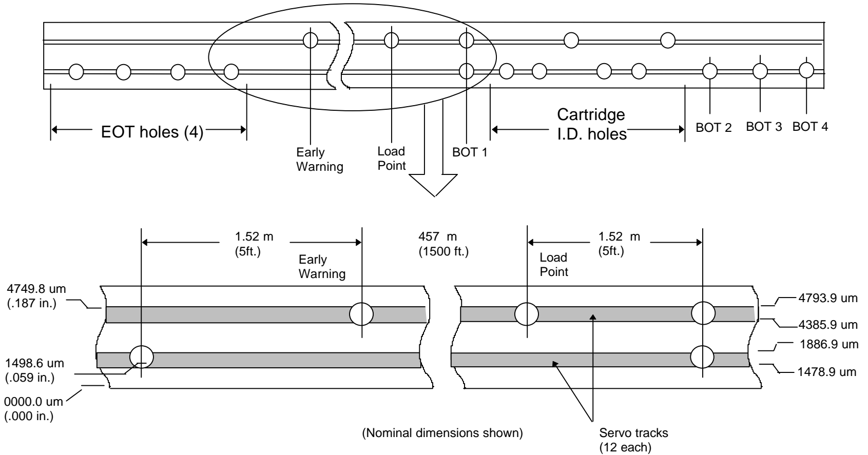
Figure A.3 Servo track / hole relationship Track pitch: 33um Center guard band: 63um
