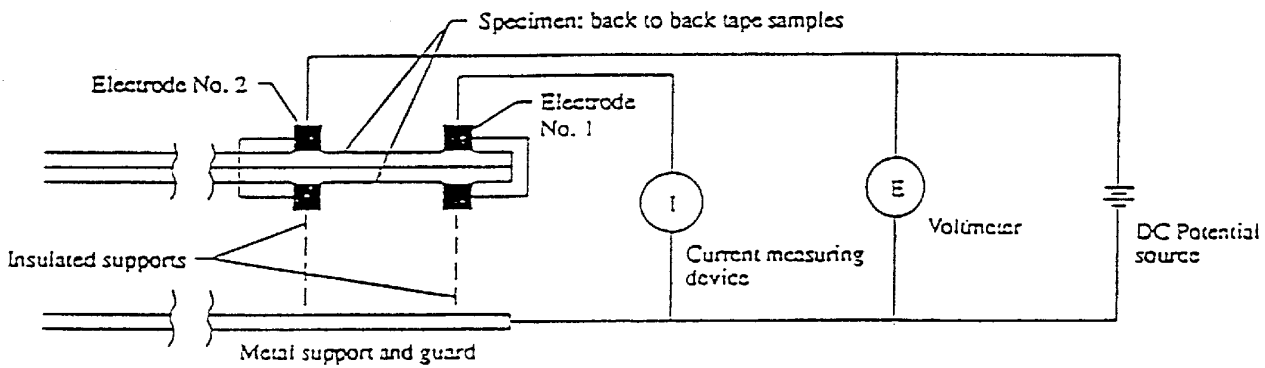
Figure 4 – Tape resistance measurement circuit
